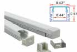
ZL-MC-1612 (-C OR -F) 4' aluminum mounting channel, Comes with 2 end caps and 2 mounting clips
